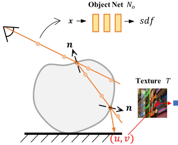
Figure 5: The illustration of our implicit refraction rendering. We locate the intersection of the ray and the implicit SDF field from the sample points and refract it twice until it hits the plane to fetch the rendered color from the plane texture.
